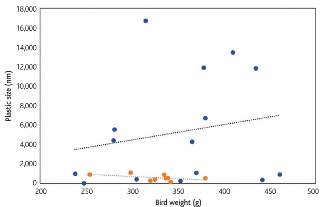
Figure 1. The average size of pieces of plastic ingested by Manx Shearwaters Puffinus puffinus , in relation to weight and age. Adults are represented by blue dots and trendline, fledglings are represented by orange dots and trendline.
